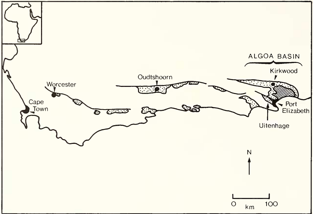
TEXT-FIG. 1. Location of Jurassic-Cretaceous sedimentary basins in the Cape Fold Belt, South Africa. The Enon and Kirkwood formations are cross-hatched, the Sundays River Formation is stippled. Modified after McLachlan and McMillan (1976).
